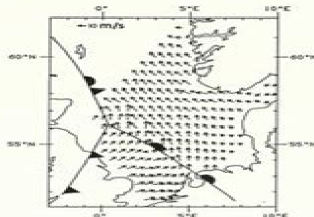
Reinterpolated wind field in North Sea on 29 September 1978.
