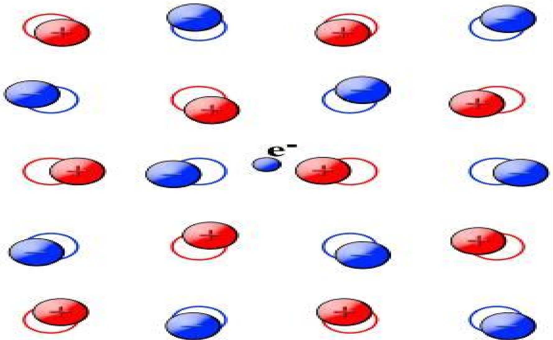
Fig. 1: Artist view of a polaron. A conduction electron in an ionic crystal or a polar semiconductor repels the negative ions and attracts the positive ions. A self-induced potential arises, which acts back on the electron and modifies its physical properties.
