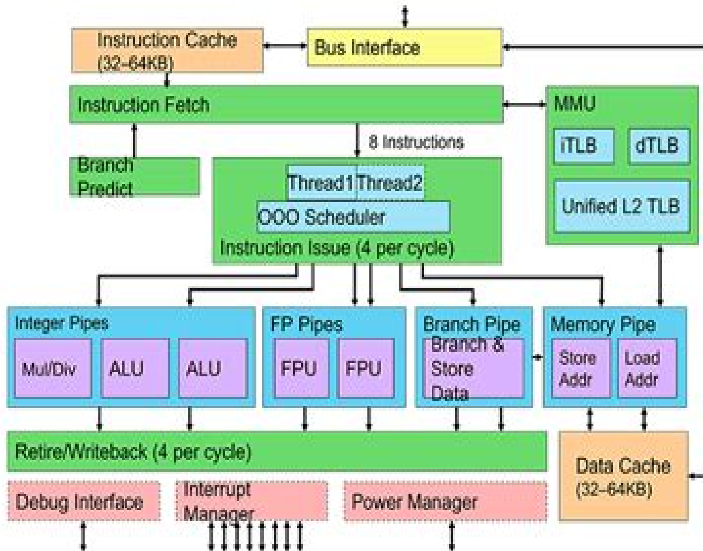
Figure 2. eVocore P8700 block diagram
