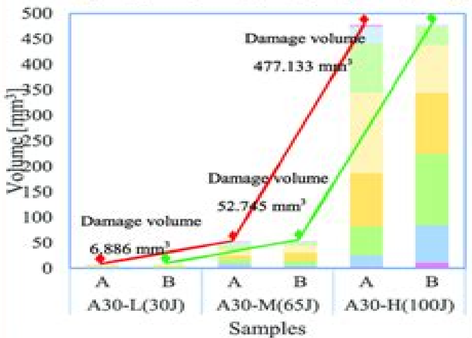
(b) Damage volume distribution diagram
