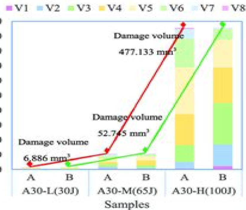
(b) Damage volume distribution diagram
