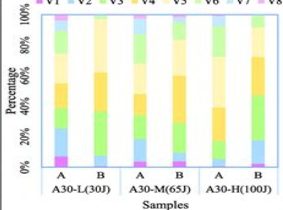
(c) Damage volume distribution percentage
