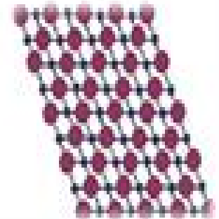
Detwinned Martensite
