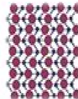
Twinned Martensite
