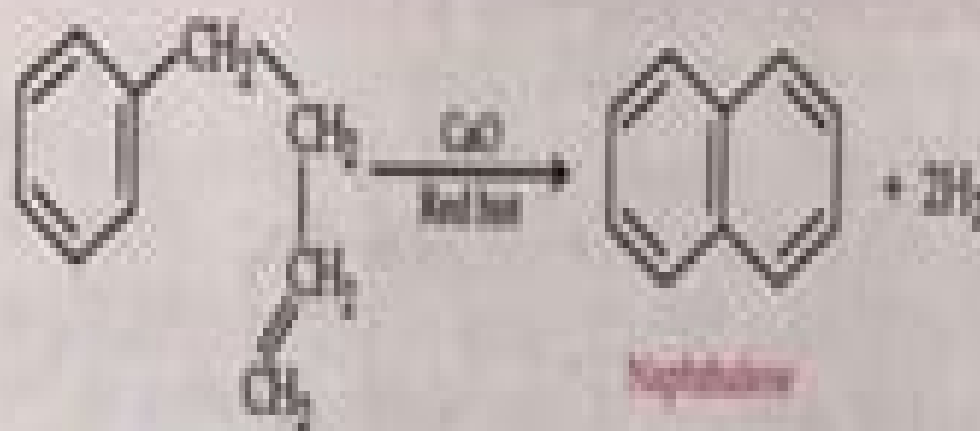
4-phenylbut-1-ene
