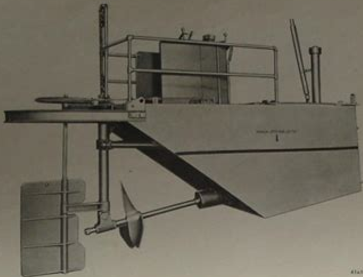
The Chrysler Sea Hole Marine Tractor, Model 4C
