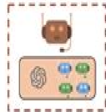
GroupChatManager
