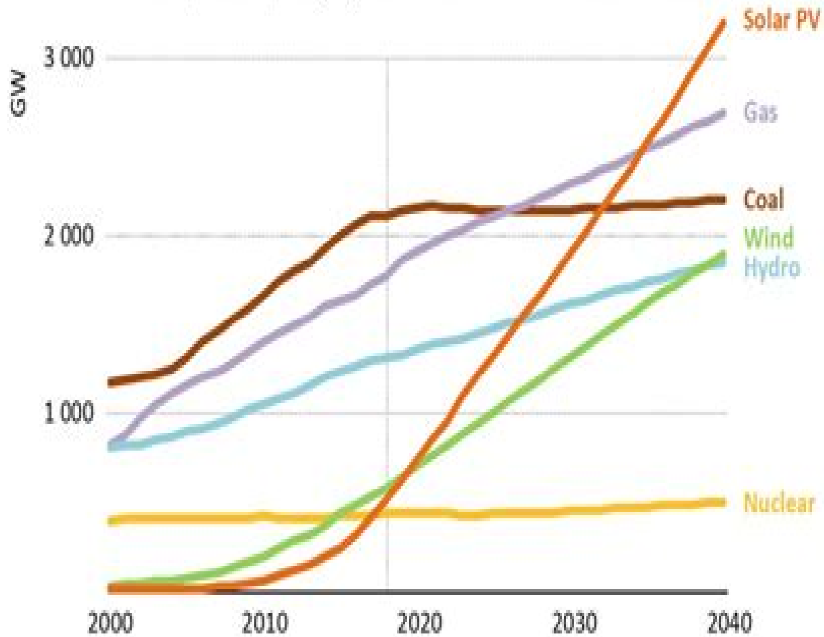
Global power capacity by source in the Stated Policies Scenario
