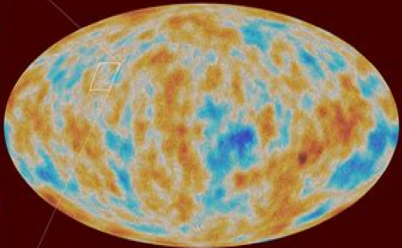
Full sky map Filtered at 5 degrees
