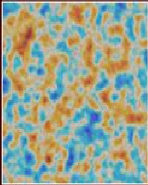
Filtered at 20 arcminutes
