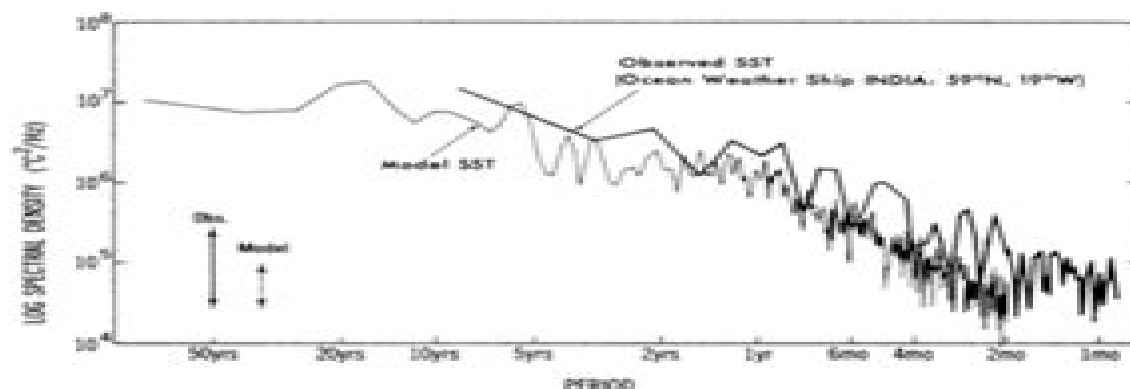
FIGURE 1 Heavy, solid line: spectrum of sea surface temperature from observed data (ocean weather ship India, 59°N, 19°W). Light, solid line: spectrum of model sea surface temperature from grid point closest to 59°N, 19°W. The arrows in the lower left corner denote 95 percent confidence intervals about the spectra. (From Delworth et al., 1993; reprinted with permission of the American Meteorological Society.)
