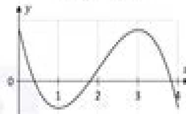
Graph of y = p(x)
