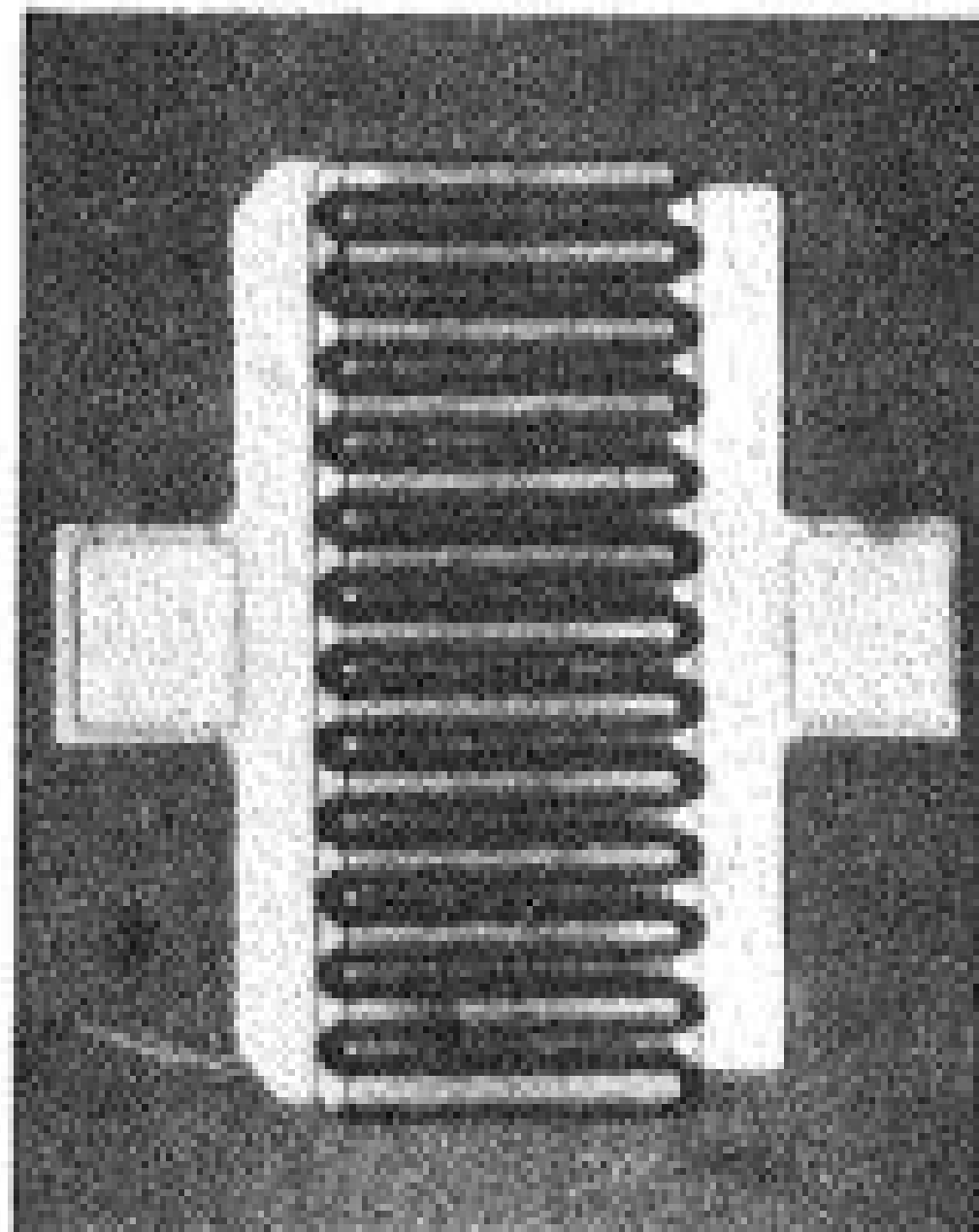
FIGURE 12-3 Geometry of an interdigitated planar microwave transistor.
