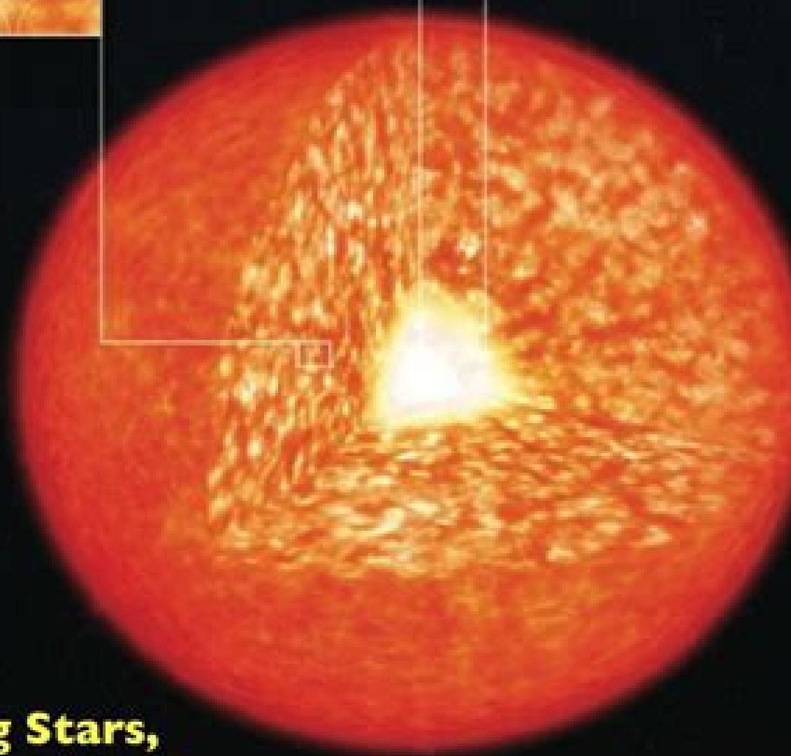
Red Giant
