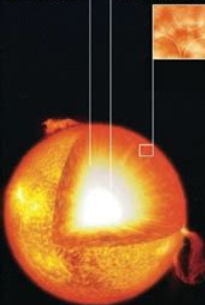
Solar type
