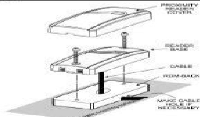
Figure 3. RDM-4 Mounting
