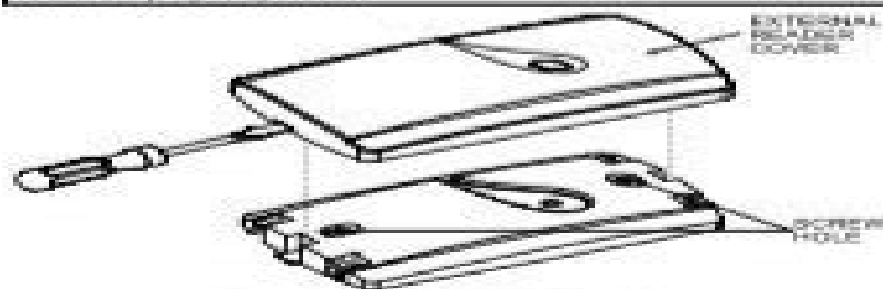
Figure 2. RDR-4, RDR-4B Mounting
