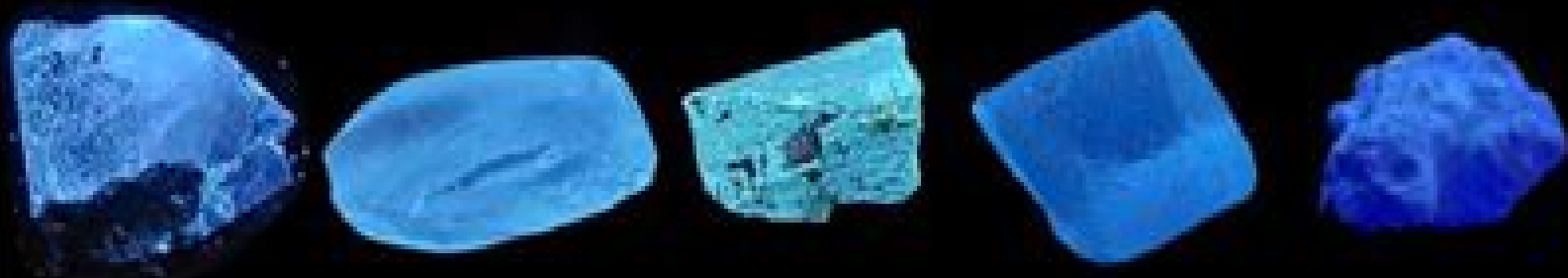
Synthetic corundum
