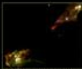
Orion Nebula This nebula is one of the most famous in the sky, located in the constellation Orion. It is a giant molecular cloud that is being ionized by the nearby stars.
