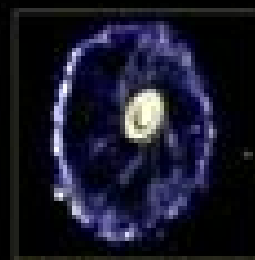
Black Hole This image shows a black hole, a region of space where the gravity is so strong that nothing can escape. The bright ring of light is the accretion disk, the material being pulled into the black hole.
