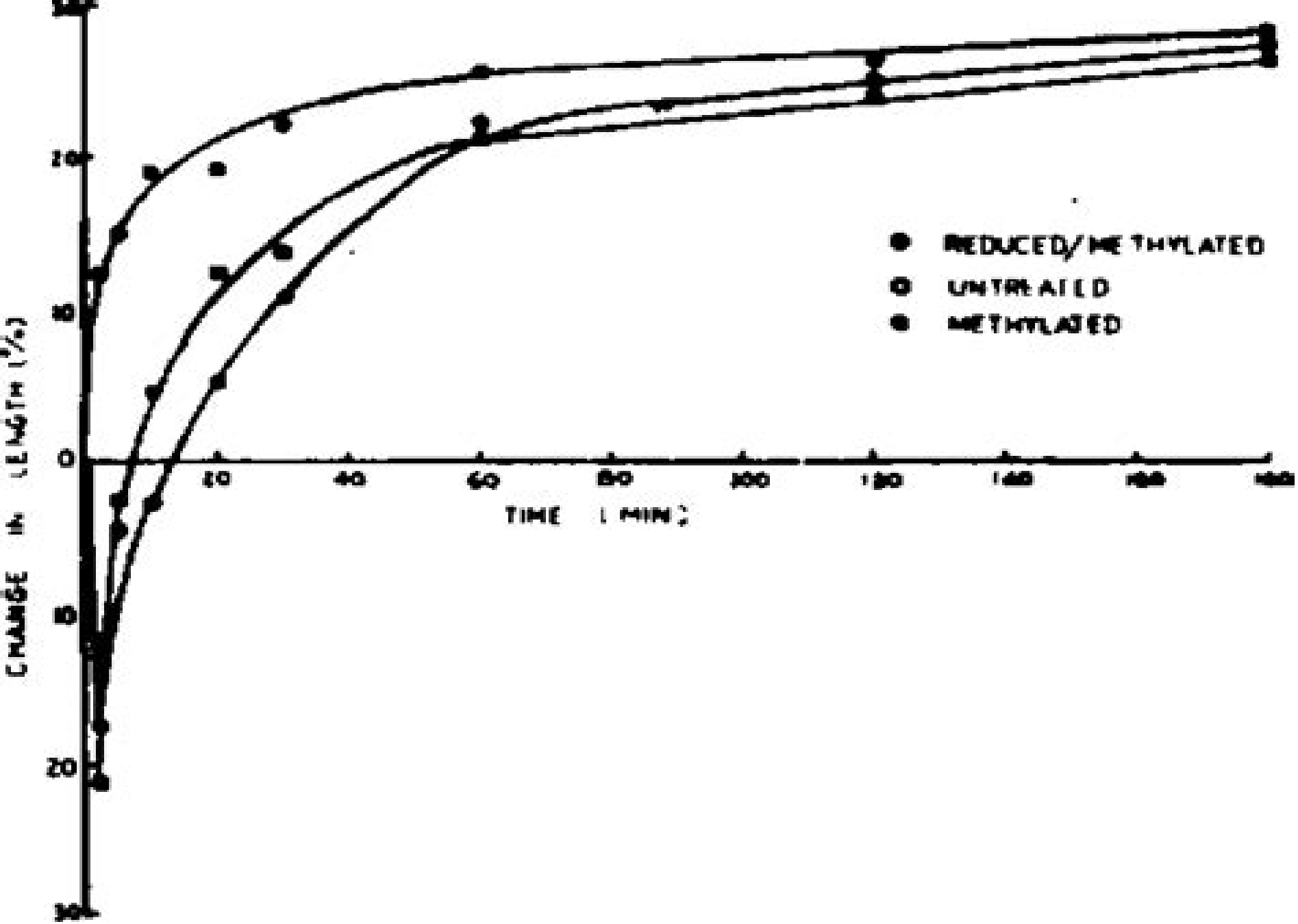
Fig. 1. Change in length in water at 100^{\circ}\text{C} for various times.
