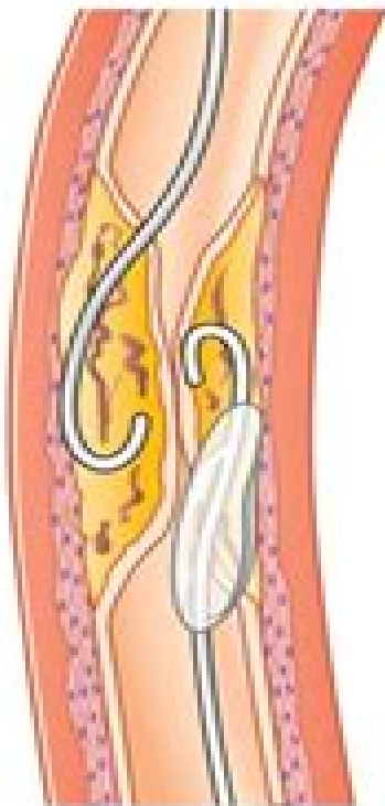
CART
