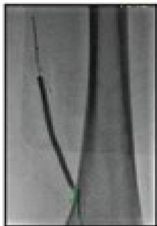
CART
