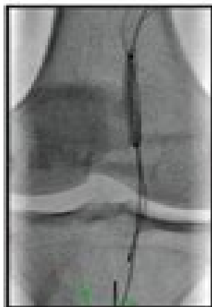
Reverse CART
