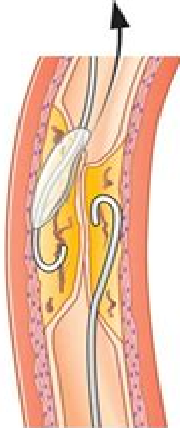
Reverse CART
