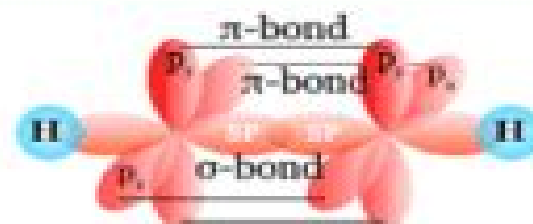
ACETYLENE
