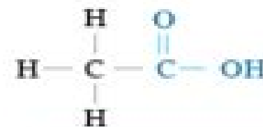
ACETIC ACID
