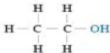
ETHANOL
