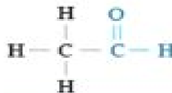
ACETALDEHYDE
