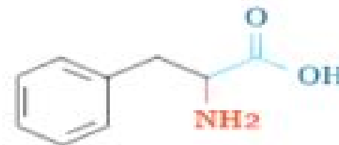
PHENYLALANINE
