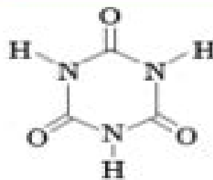
CYANURIC ACID
