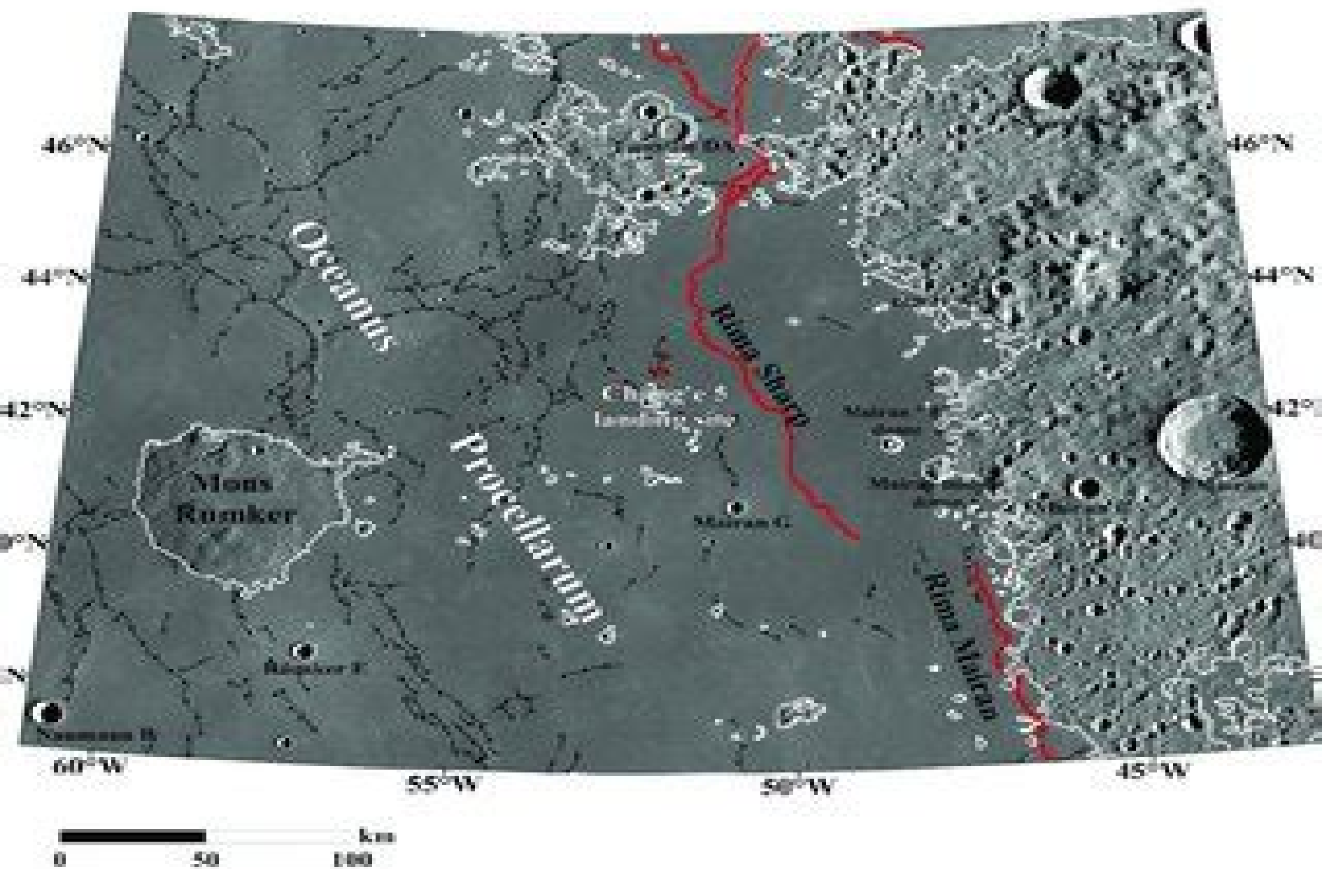
Figure 1. Context of the CE-5 samples return region. The background is a mosaic of TC morning data (B
