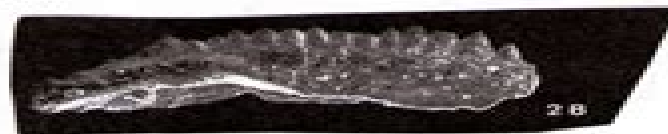
Figure 8. Flajisella species and a related form; all figures \times 40 . 1–4, Flajisella schulzei (Bardashev), TO-I 17 I/1. 5, 6, " Ozarkodina " excavata (Branson and Mehl), TO-I 17 I/2. 7–22, F. schulzei ; 7–9, TO-I 17; 10–13, COP-IV 197 II/5; 14–16, TO-I 18 I/6; 17–19, TO-I 18 I/5; 20–22, TO-I 18 I/4. 23–25, F. sigmoidostygia n. sp., TO-I 18 I/3. 26–28, F. spolia (Flajis), TO-I 23 I/3. 29–33, F. pigmostygia n. sp., TO-I 20 I/49, I/50. 34–36, F. laevis (Bardashev), TO-I 23 I/1.
