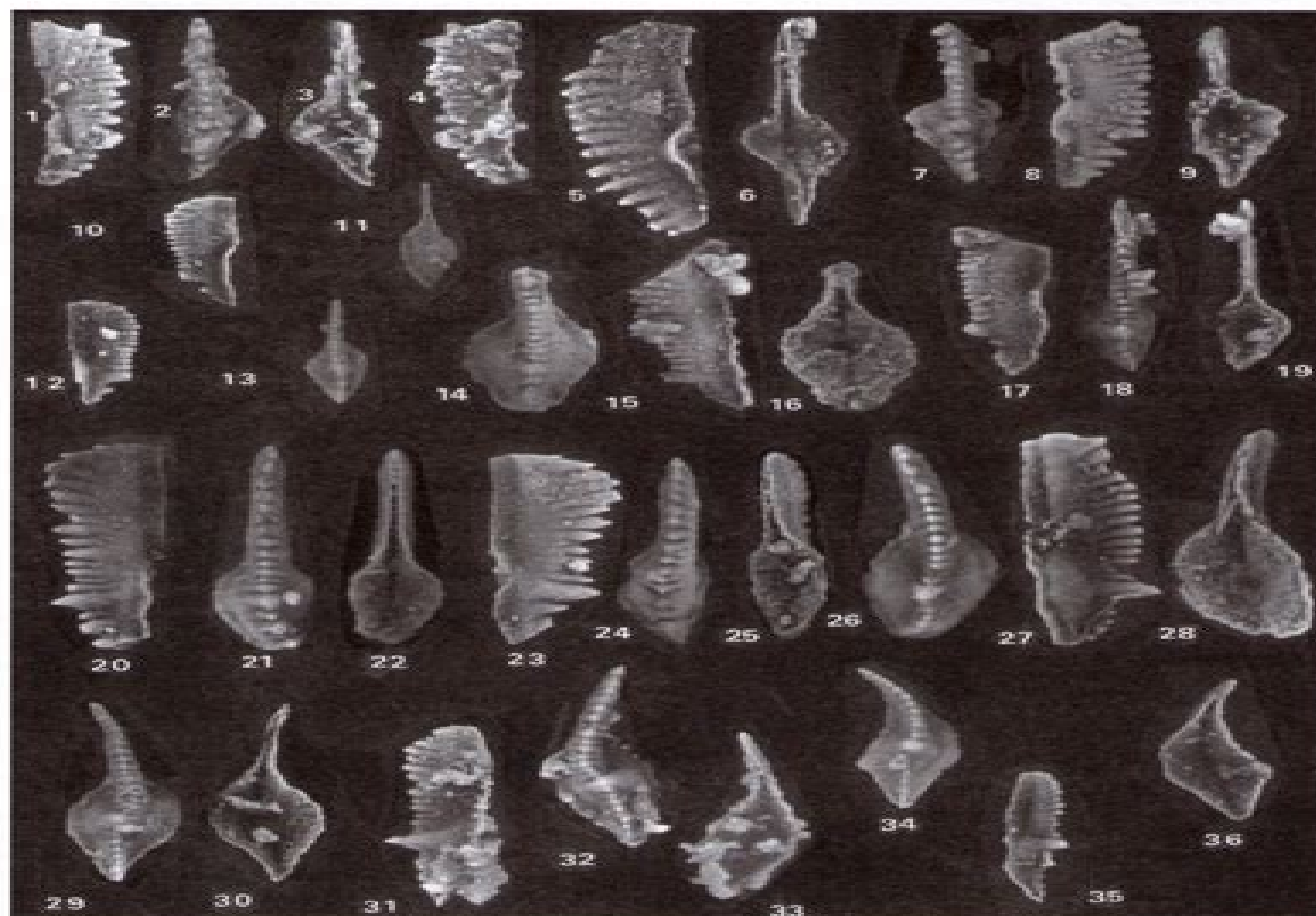
Figure 8. Flajisella species and a related form; all figures \times 40 . 1–4, Flajisella schulzei (Bardashev), TO-I 17 I/1. 5, 6, " Ozarkodina " excavata (Branson and Mehl), TO-I 17 I/2. 7–22, F. schulzei ; 7–9, TO-I 17; 10–13, COP-IV 197 II/5; 14–16, TO-I 18 I/6; 17–19, TO-I 18 I/5; 20–22, TO-I 18 I/4. 23–25, F. sigmoidostygia n. sp., TO-I 18 I/3. 26–28, F. spolia (Flajis), TO-I 23 I/3. 29–33, F. pigmostygia n. sp., TO-I 20 I/49, I/50. 34–36, F. laevis (Bardashev), TO-I 23 I/1.
