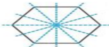
Regular Hexagon 6 lines of symmetry
