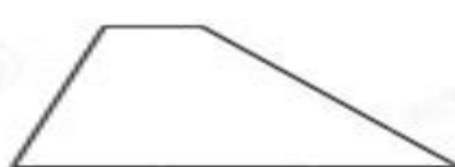
Trapezoid No lines of symmetry
