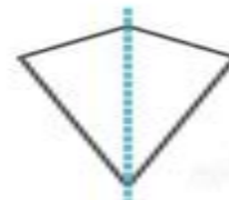
Kite 1 line of symmetry
