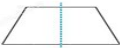
Isosceles Trapezoid 1 line of symmetry
