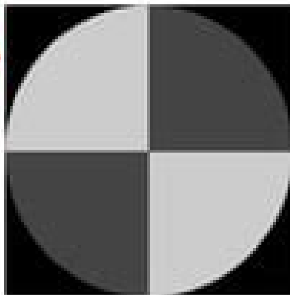
Recovered albedo
