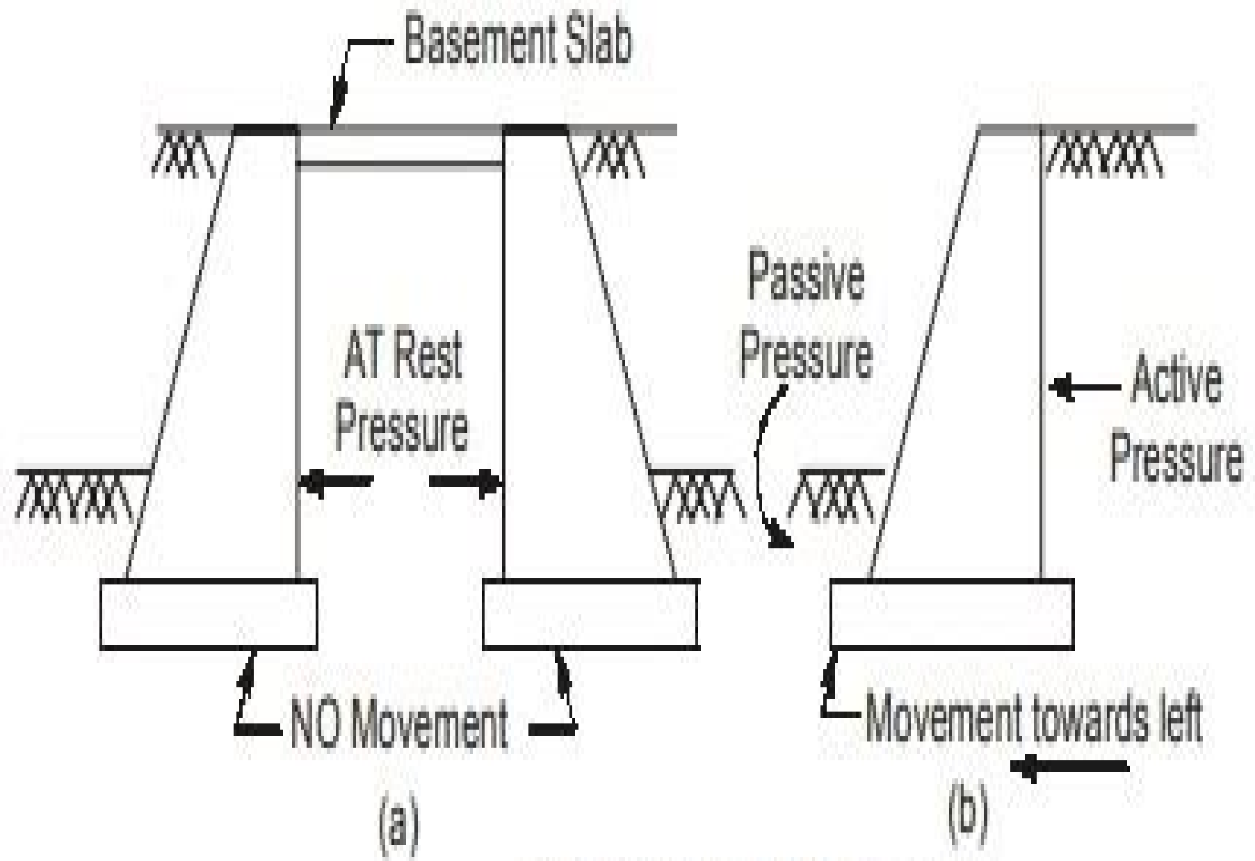
Fig: Types of Earth Pressure
