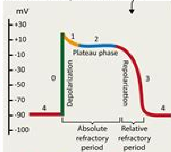
Contractile myocardium
