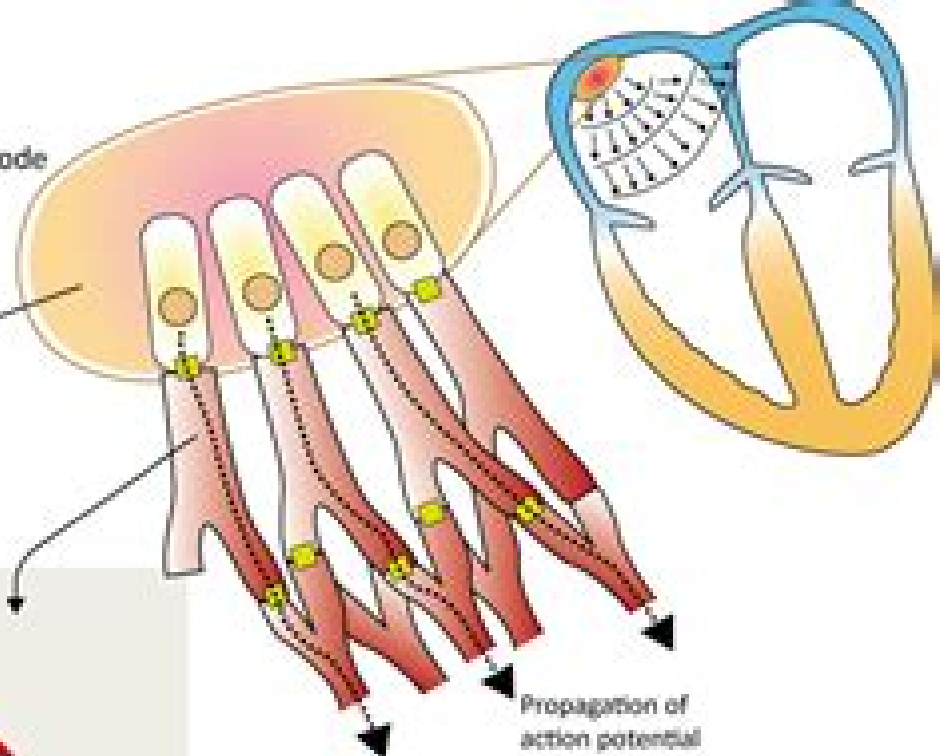
■ = Gap junction
