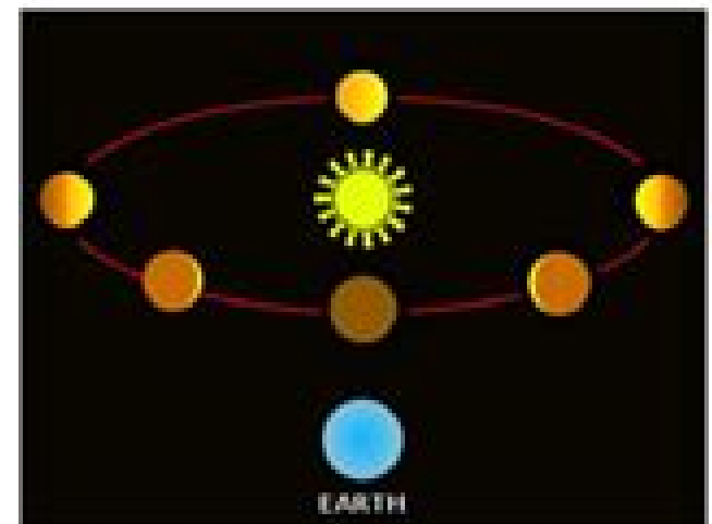
Phases of Venus: Size would be constant in a geocentric system.
