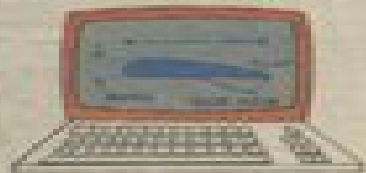
closed sub-routine
