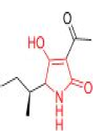
tenuazonic acid
