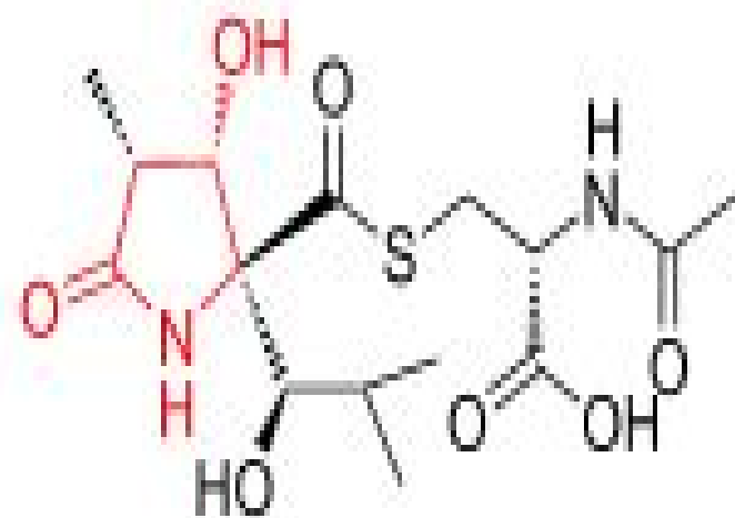
lactacystin
