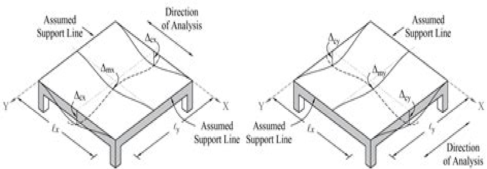
a) X Direction Bending
