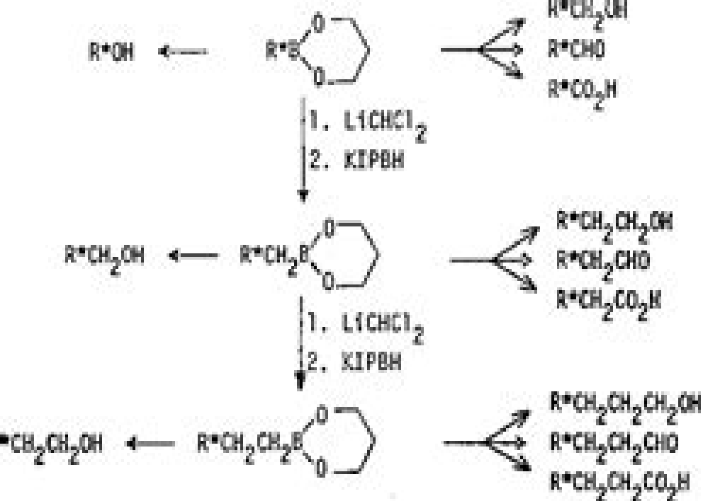
Fig. 45. Synthesis of optically active derivatives via successive homologations
