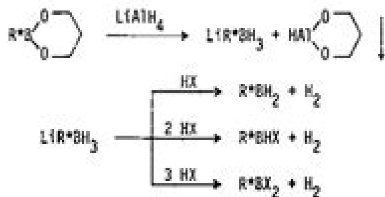
Fig. 46. Conversion of optically active boronic acids into optically active borohydrides and derived boranes
