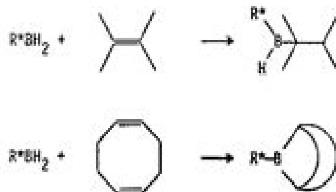
Fig. 47. Synthesis of optically active thexyl and 9-BBN derivatives
