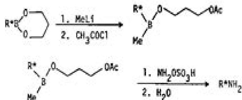
Fig. 48. Procedure for the synthesis of primary amines in high enantiomeric purity
