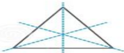
Equilateral Triangle 3 lines of symmetry
