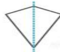
Kite 1 line of symmetry
