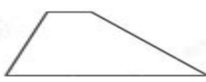
Trapezoid No lines of symmetry
