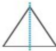
Isosceles Triangle 1 line of symmetry
