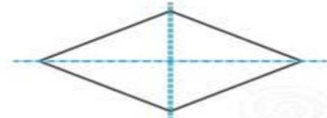
Rhombus 2 lines of symmetry
