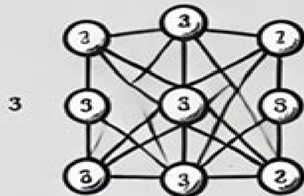
COMPLETE GRAPH
