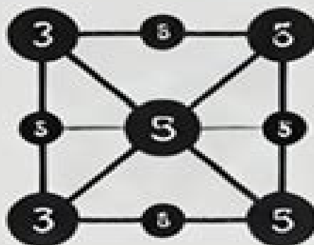
SIMPLE GRAPH
