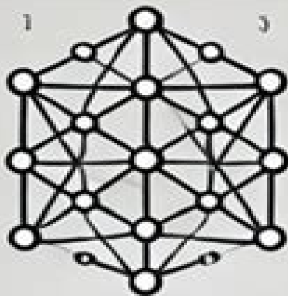
UNDIRECTED GRAPH
