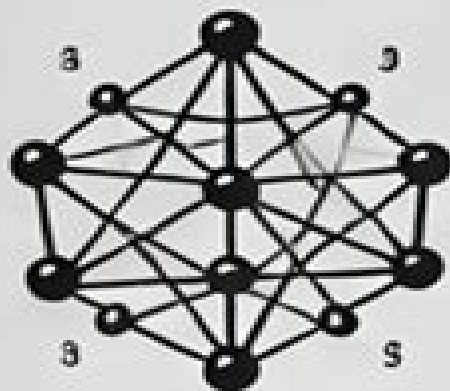
SIMPLE GRAPH
