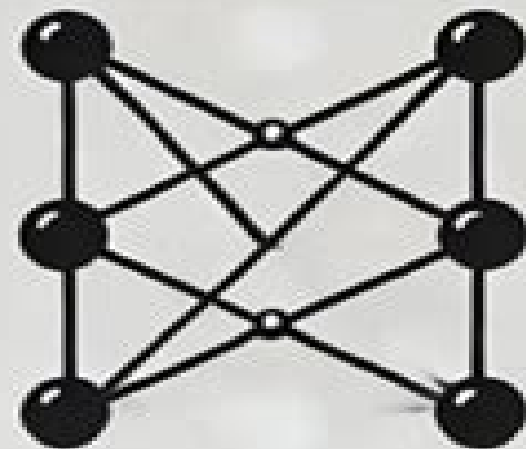
DIRECTED GRAPH
