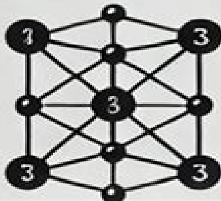
SIMPLE GRAPH
