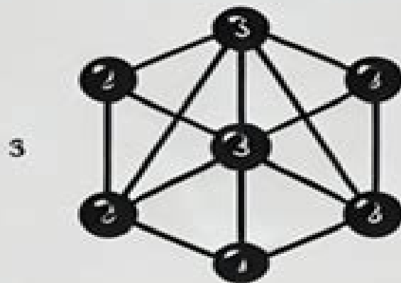
SIMPLE GRAPH
