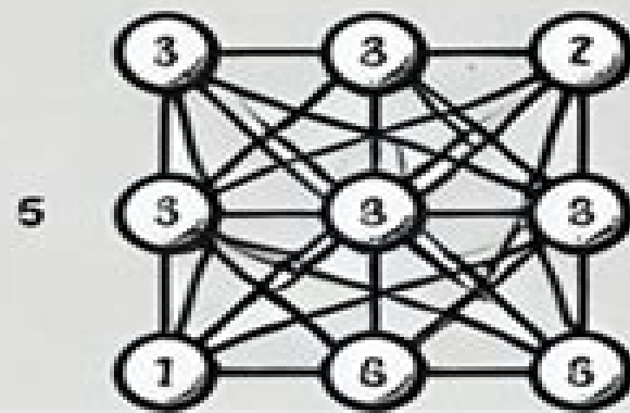
COMPLETE GRAPH
