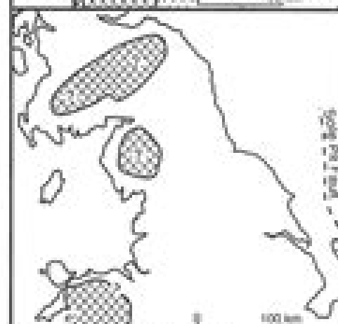
(b) Early Carboniferous (mid Dinantian)
