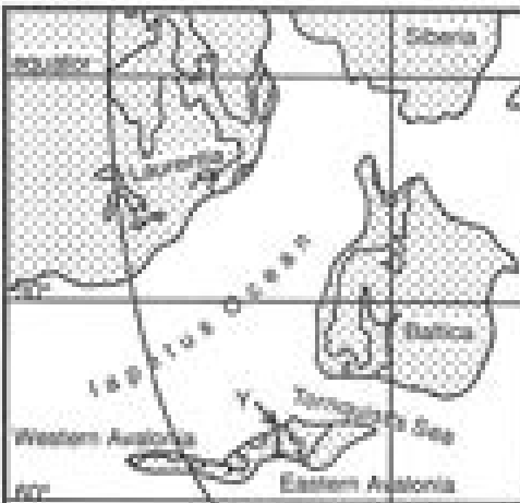
(a) Mid Ordovician
