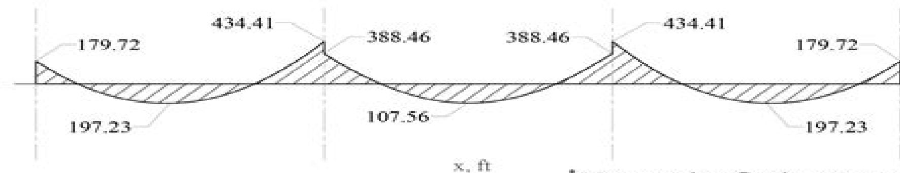
Moment diagram (ft-kips)
