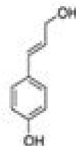
p-coumaryl alcohol
