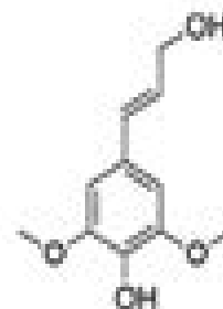
sinapyl alcohol
