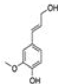
coniferyl alcohol
