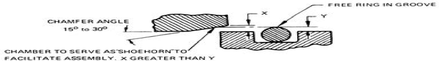
Figure 4. Chamfer piston for rod gland
