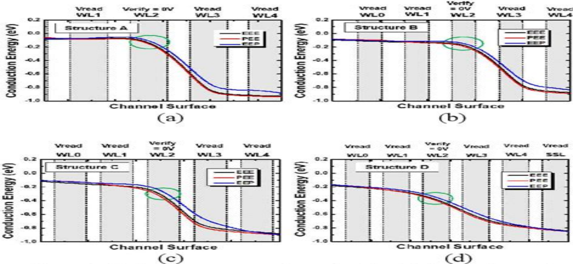
Figure 4. Conduction energy at channel surface during read operation (a) structure A, (b) structure B, (c) structure C, (d) structure D.
