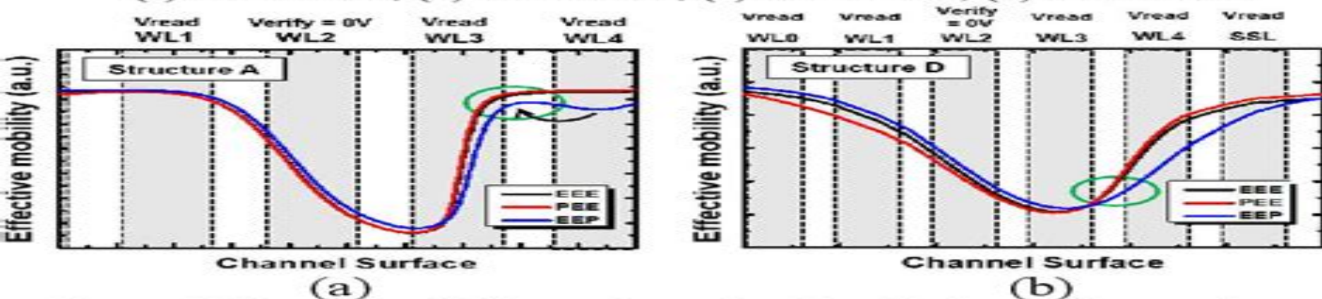
Figure 5. Electron mobility at channel surface during read operation (a) structure A, (b) structure D.
