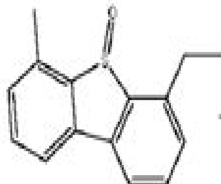
4-ethyl-6-methyl-dibenzothiophene 3-oxide
