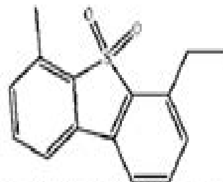
4-ethyl-6-methyl-dibenzothiophene 3,3-dioxide
