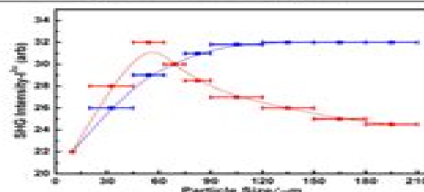
Figure 1. Phase-matching (blue) and nonphase-matching (red) curves for powder SHG measurements.
