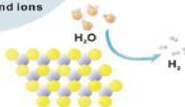
Hydrogen evolution reaction
