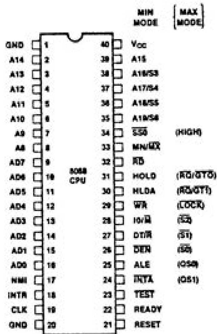
Figure 2. 8088 Pin Configuration
