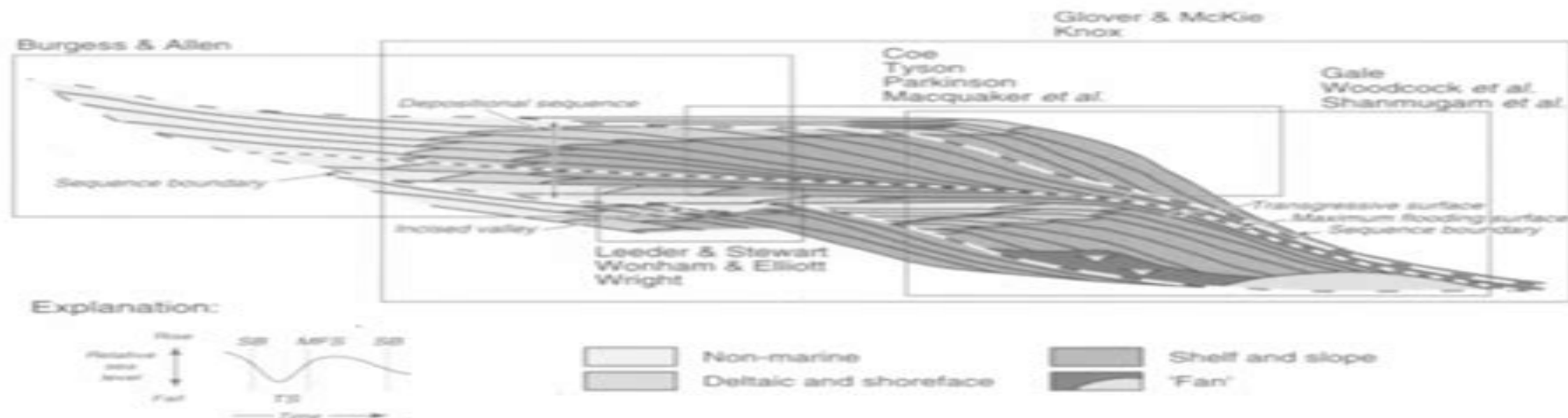
Fig. 1. The standard sequence stratigraphical model for siliciclastic systems (based on Haq et al. 1988 and Christie-Blick & Driscoll 1995) showing the different areas covered by papers in this volume. Wright (this volume) and Coe (this volume) discuss successions that were carbonate ramps, with an implied sequence stratigraphical character not dissimilar to siliciclastic deposits (see Schlager 1992; Tucker et al. 1993). A sequence boundary (SB) is defined as an unconformity and its basinward correlative conformity. The lower of the sequence boundaries in this figure ( type 1 ) is distinguished from the upper one ( type 2 ) by its association with 'fan' sedimentation at the toe of slope, which has been related to rapid, high-magnitude, relative sea-level fall. The maximum flooding surface (MFS) corresponds to the time of greatest landward extent of the facies belts within a depositional sequence, and is characterized by detrital sediment starvation in basinward regions. The transgressive surface (TS) is a widespread horizon across which deep-water sediments abruptly overlie shallow water sediments, and it forms as the underlying progradational sedimentary succession is flooded by rising relative sea level. Systems tracts are defined between these key surfaces. For full discussion of this model, definition of systems tracts and their relation to relative and eustatic sea-level change the reader should refer to Haq et al. (1988), Posamentier & Vail (1988), Posamentier et al. (1988, 1990, 1992), Mitchum & Van Wagoner (1991), Vail et al. (1991), Jacquin et al. (1992) and Posamentier & James (1993). Useful critiques and alternative models are provided by Miall (1986), Galloway (1989), Carter et al. (1991), Fulthorpe (1991), Schlager (1991), Walker (1992) and Christie-Blick & Driscoll (1995), and references therein. As a substitute for depositional sequences as defined above, Galloway (1989) has proposed use of genetic stratigraphic sequences bounded by maximum flooding surfaces, and his approach has also been followed by many workers.
