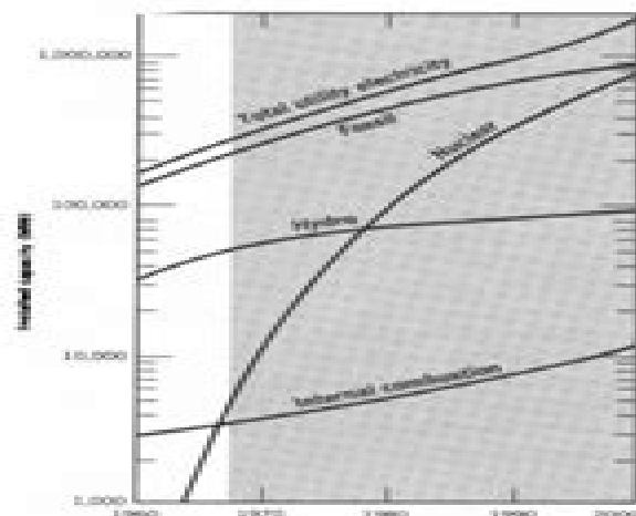
FIGURE 16 Projection to the year 2000 showing the increasing importance of nuclear fuels for generating utility electricity. [Reprinted from Environmental Science and Technology , June 1967, page 468, with permission of the American Chemical Society.]
