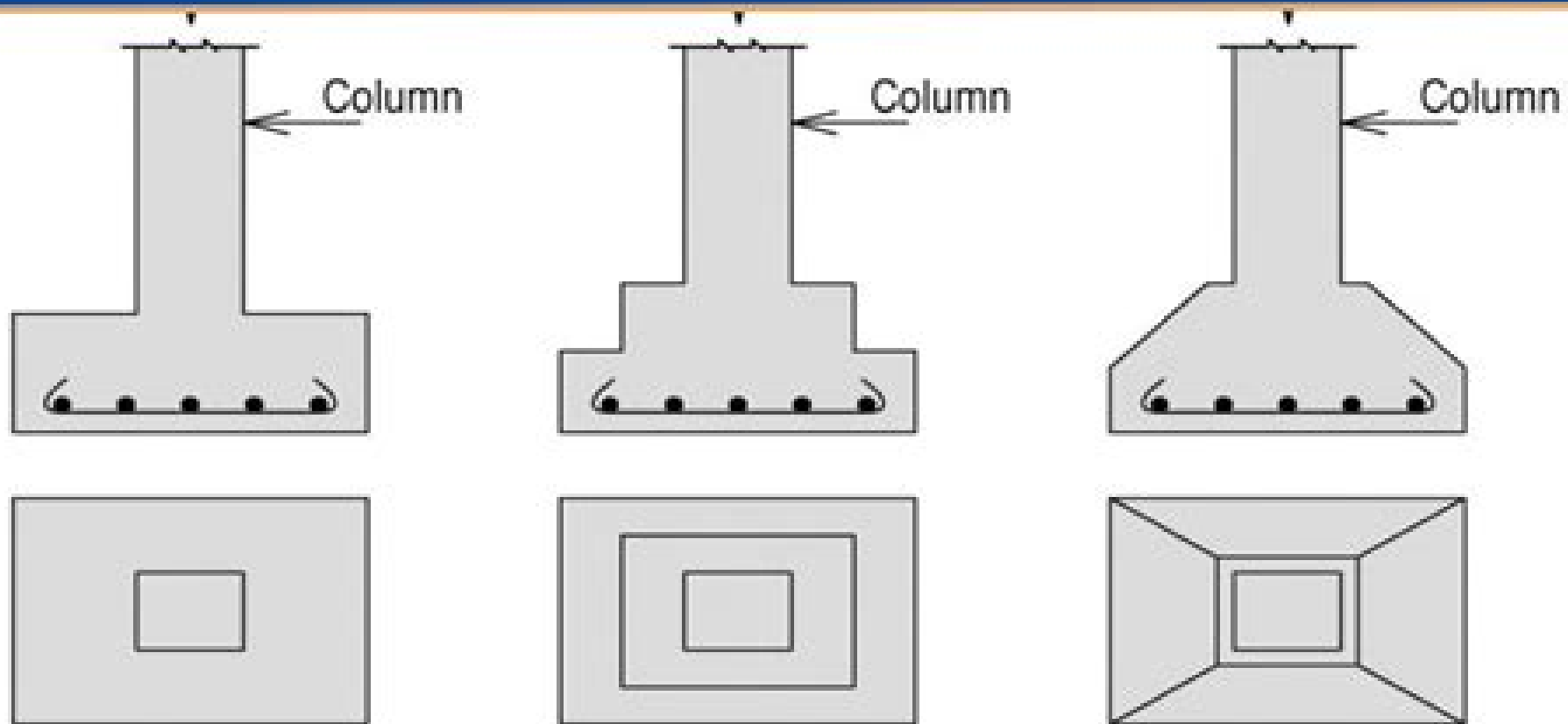
Shallow Foundation
