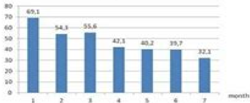
Average total score
