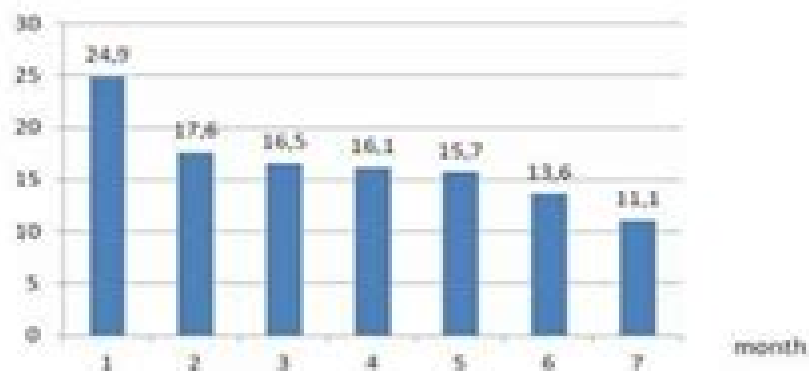
Average score of hyperactivity
