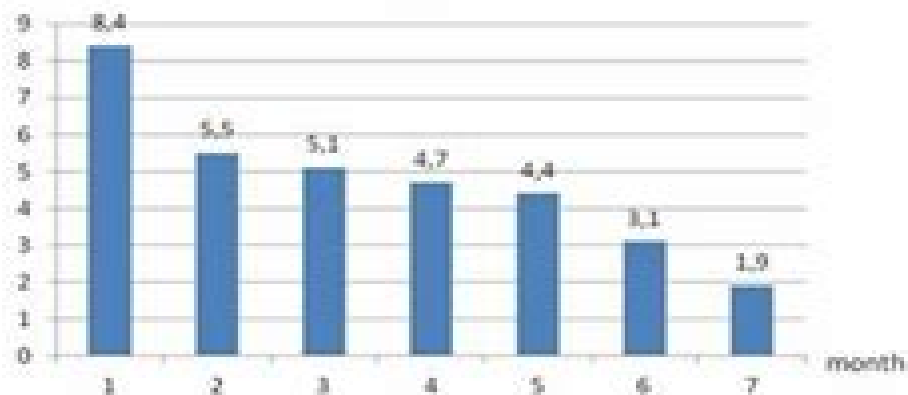
Total score of speech disorders
