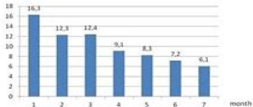
Total score of irritability
