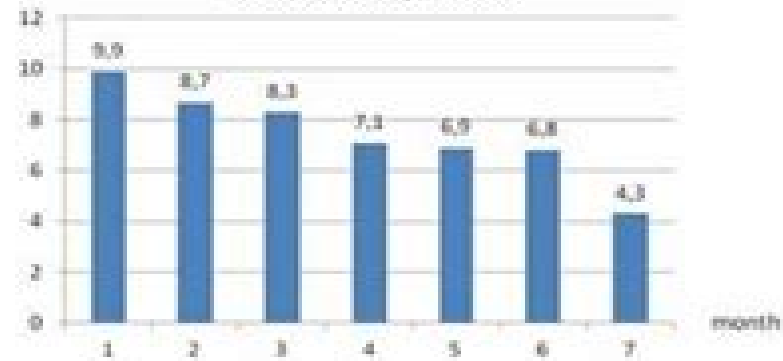
Total score of eye contact
