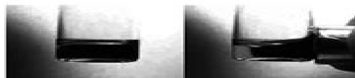
Fig. 1. Pictures showing the response of bmim[FeCl 4 ] to a small Nd magnet (0.55 T) [7]. In order to show the displacement and distortion of bmim[FeCl 4 ] more clearly, water is added to the sample liquid. Left: two layers of liquids, water (upper) and bmim[FeCl 4 ] (lower), are seen when no magnetic field is applied. Right: bmim[FeCl 4 ] is attracted and moves toward the magnet and the liquid is distorted to a concave shape.
