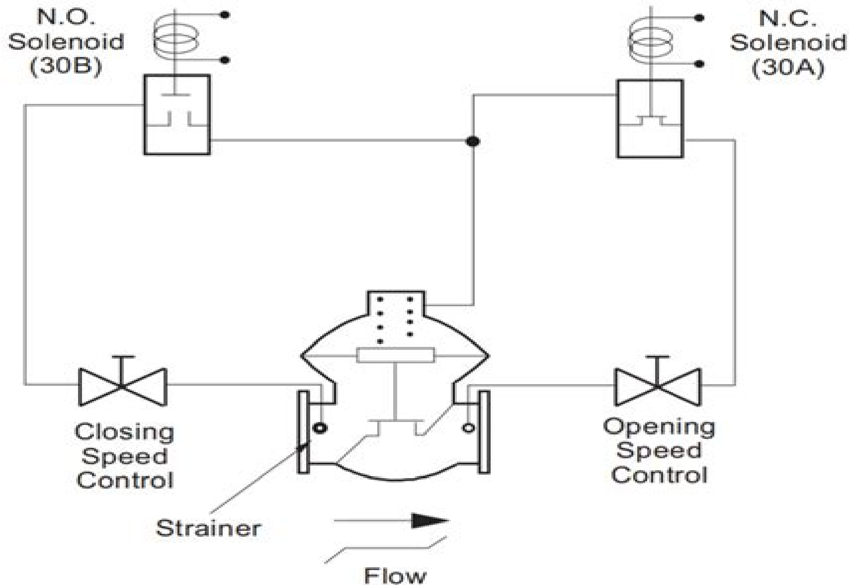
Model 210 Valve Schematic
