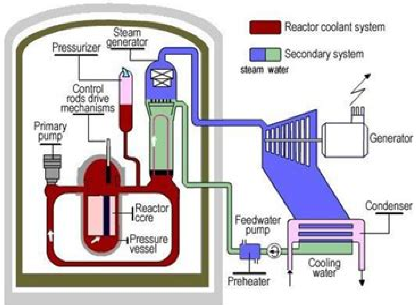
Schematic View of PWR
