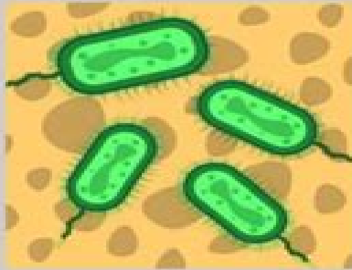
Bacteria
