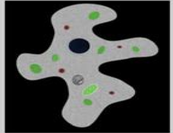
Amoeba
